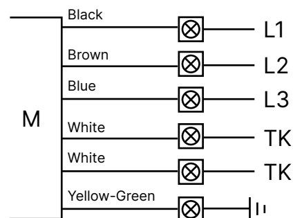
Y-connection
