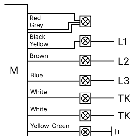
Y-connection
