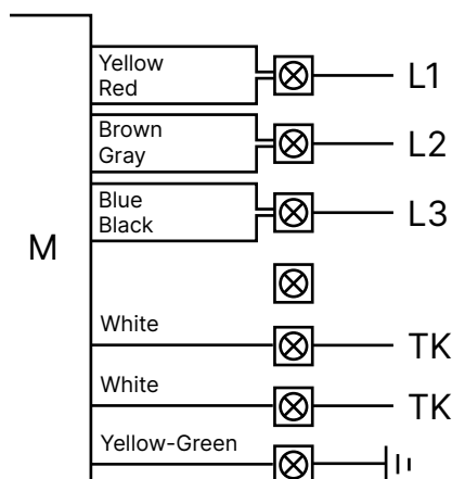
Δ-connection
